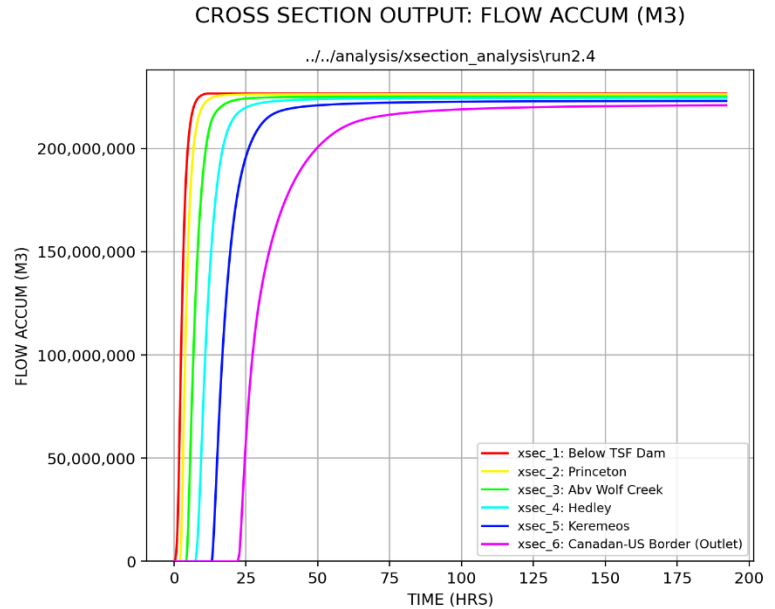
Figure 3-6: Accumulated flow at six cross sections for the 12-hour, 40% breach scenario of the expanded TSF in the 30 m model
