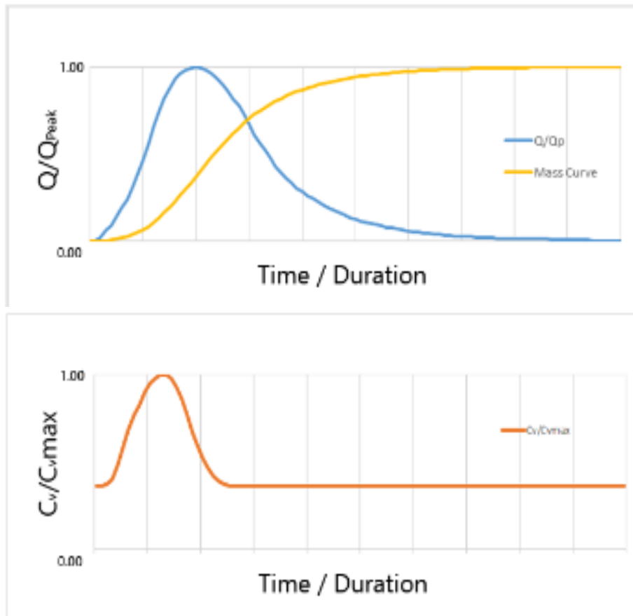
Figure 3-5. FLO-2D default breach hydrograph (top) and sediment concentration curves (bottom).
