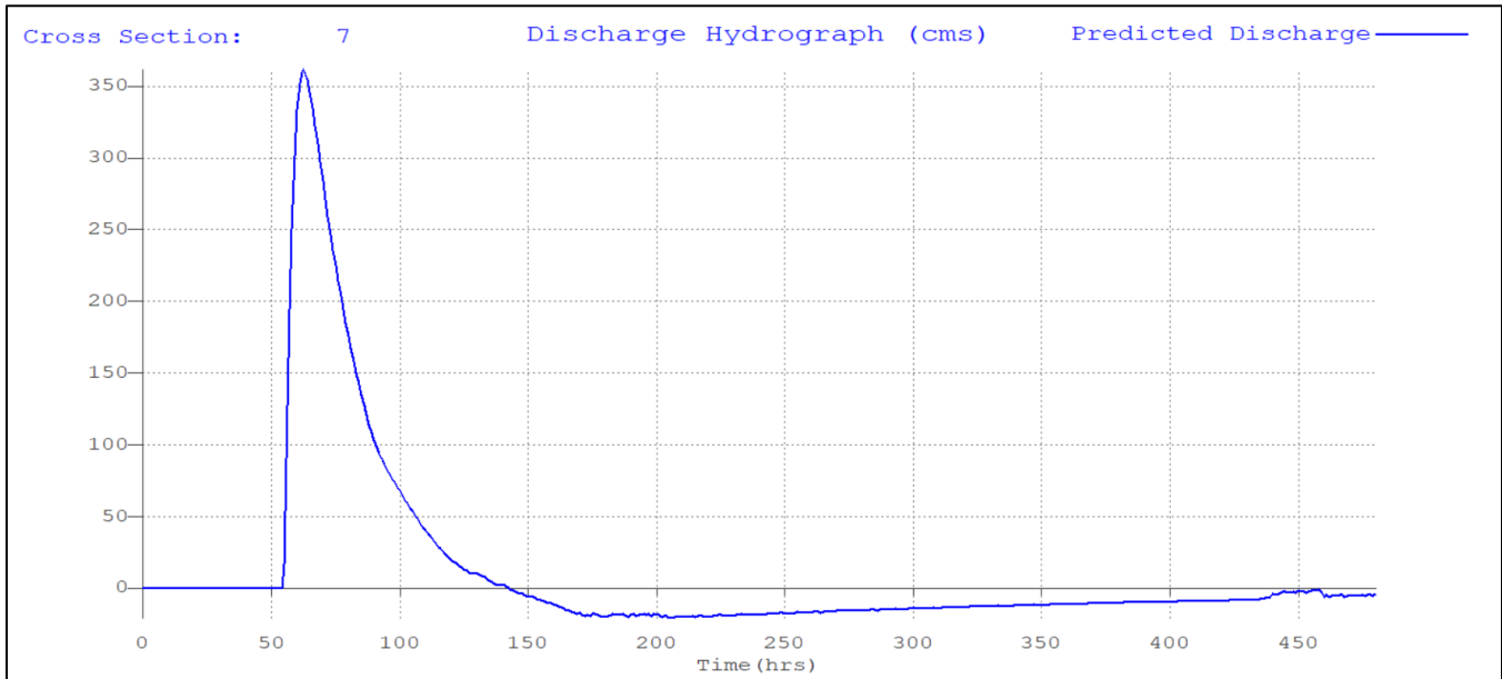
A 22: Hydrograph at the cross-section below Lake Palmer, WA showing the debris flow into the lake around hour 60-70, followed by the outflow of the displaced water back downstream into the Similkameen River, as denoted by the negative flows from hour 150 onward. Default 40% breach scenario for the permitted CMM TSF.
