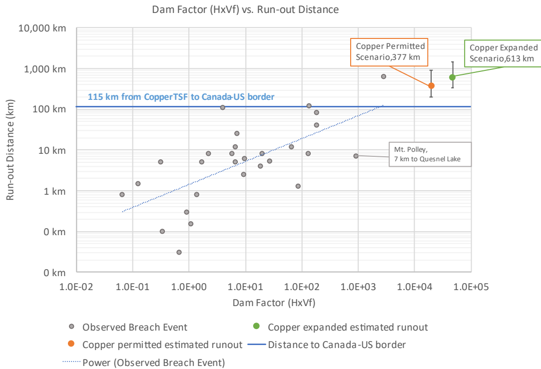
Figure 2-3. Comparison of dam factor and observed breach run-out distance for historical breach events (historical breach data obtained from Larrari & Lall, 2018) and the estimated Copper TSF run-out distance. Blue horizontal line shows distance to US-Canada border for reference. Note that the Mount Polley runout distance was terminated by a downstream lake.
