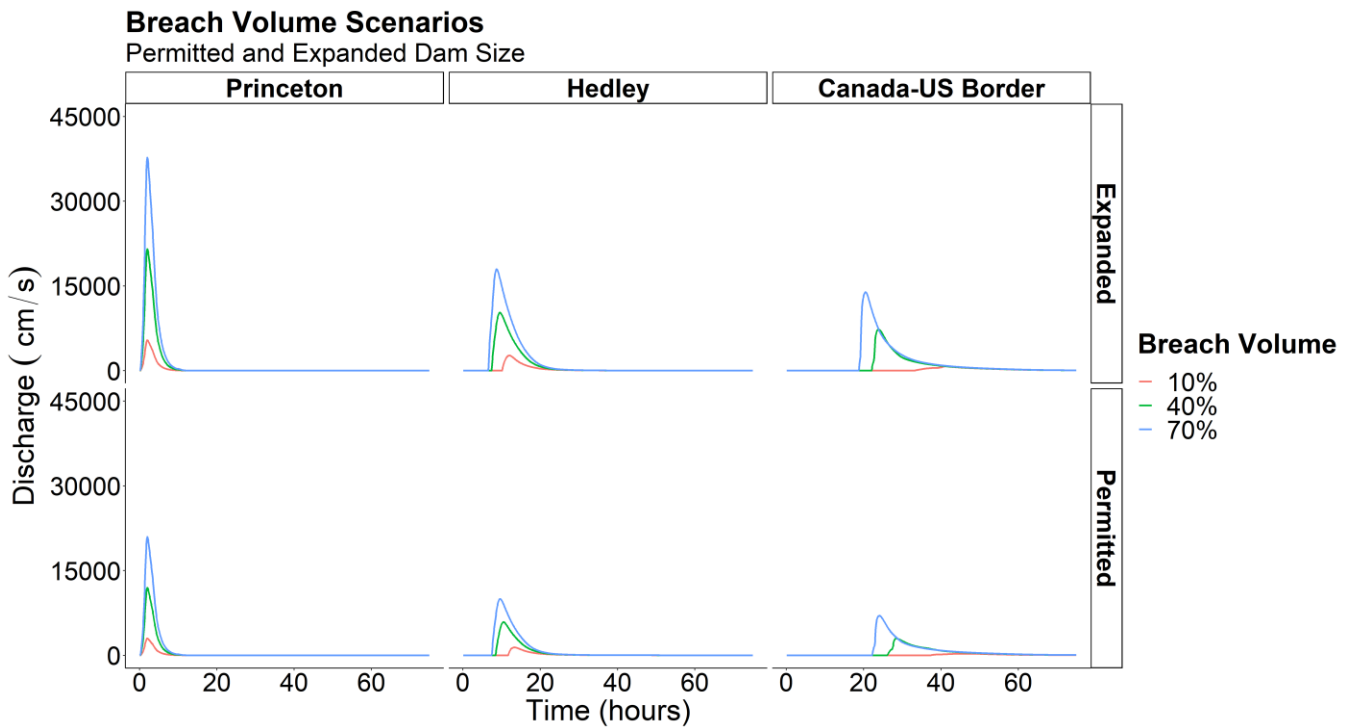
A 3. Timeseries hydrographs of low (10%), middle (40%), and high (70%) breach volumes at three cross sections along the Similkameen for the permitted dam (bottom row) and expanded dam (top row) in cubic meters per second.
