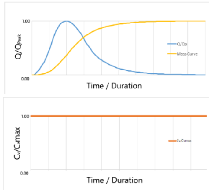
A 9. Alternative hydrograph and sediment concentration composition timeseries evaluated in model scenarios.
