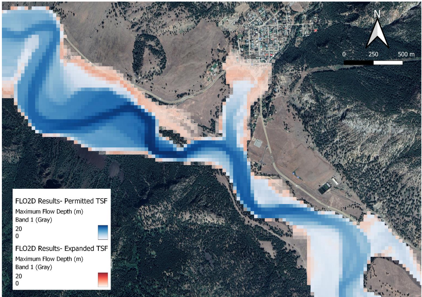
Figure 5-2: An overlay of maximum flow depths (m) in Hedley, BC from a 40% breach, 12 hour duration scenario for the permitted TSF (250 Mm 3 ; in blue colorbar) and the expanded TSF (450 Mm 3 ; in red colorbar)
