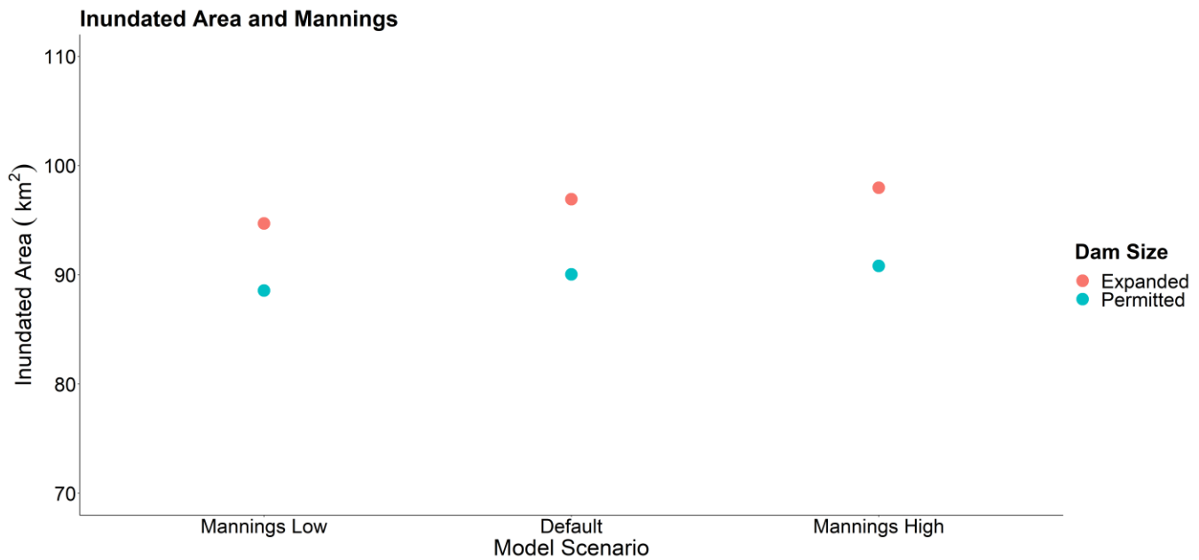
A 12. Manning’s model scenarios for both the permitted (blue) and expanded (red) dam sizes. Manning’s n values range from 50% lower to 50% higher.
