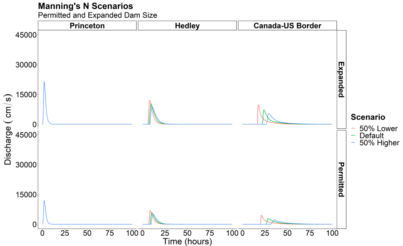
A 13. Timeseries hydrographs of low, middle, and high manning's n vales at three cross sections along the Similkameen for the permitted dam (bottom row) and expanded dam (top row) in cubic meters per second (CMS) Hydrographs are nearly identical at Princeton in both dam size scenarios.
