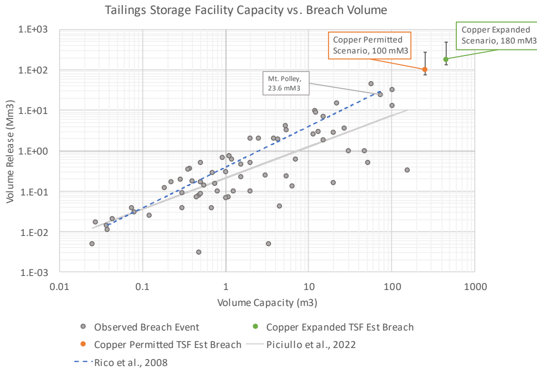
Figure 2-2. Comparison of tailings storage facility capacity and observed release volumes for historical breach events. Calculated release volume scenarios used in this study (orange and green points) are derived from the Rico et al., (2008) regression line, since Piciullo et al. (2022) was published concurrent with our modeling efforts.
